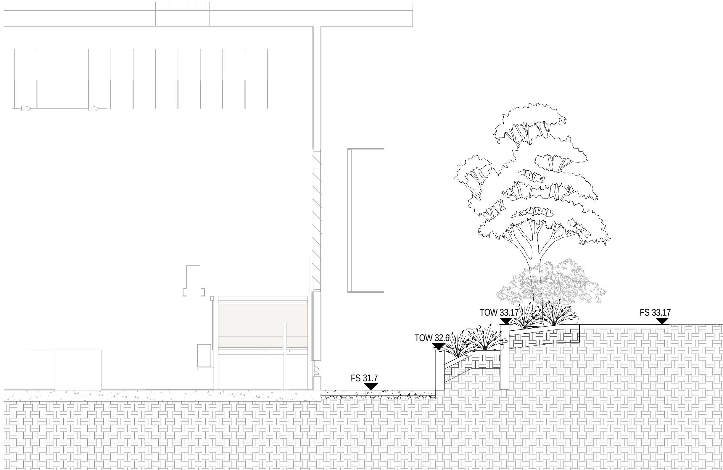
1 Section 1 LANDSCAPE SECTION - 1 : 50
